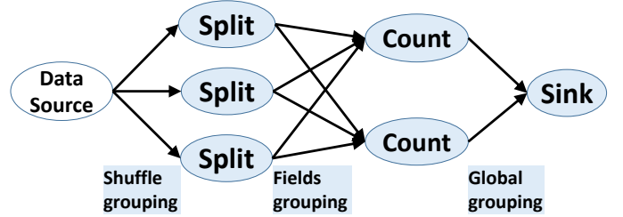
Fig. 4: Word-count execution graph.
