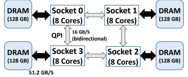
Fig. 2: NUMA topology and peak bandwidth of our sever. work in Section VII and conclude in Section VIII.
