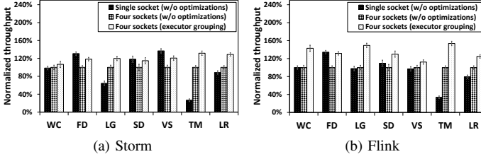
Fig. 14: NUMA-aware executor placement.
