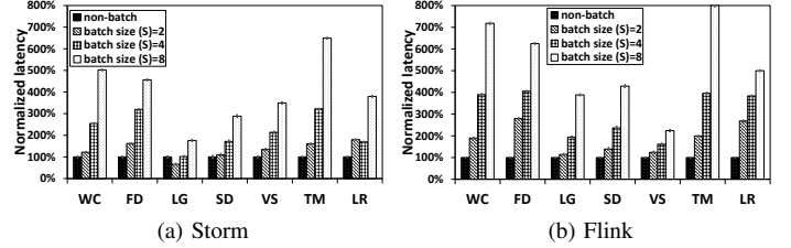
Fig. 13: Normalized latency of tuple batching optimization.
