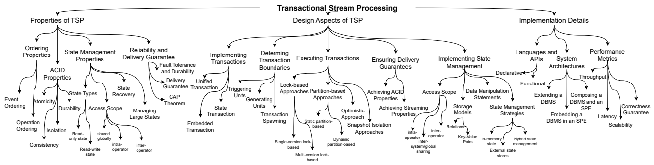
Fig. 3: Taxonomy of TSP.
