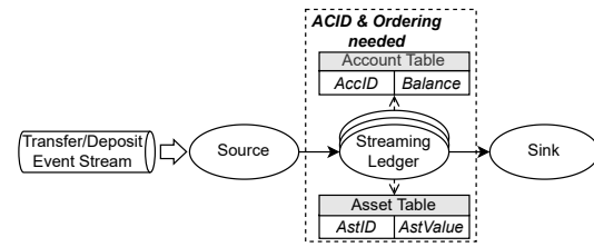
Fig. 2: Streaming Ledger (SL) [3].
