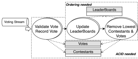
Fig. 1: Leaderboard Maintenance (LM) [54].
