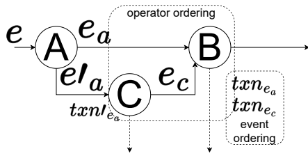
Fig. 4: Example of timestamp assignment dilemma.
